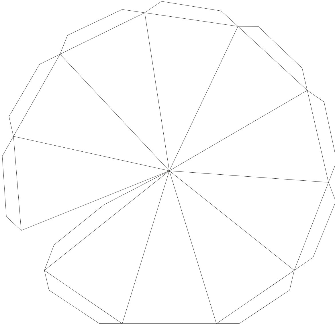
Decagonal Pyramid
