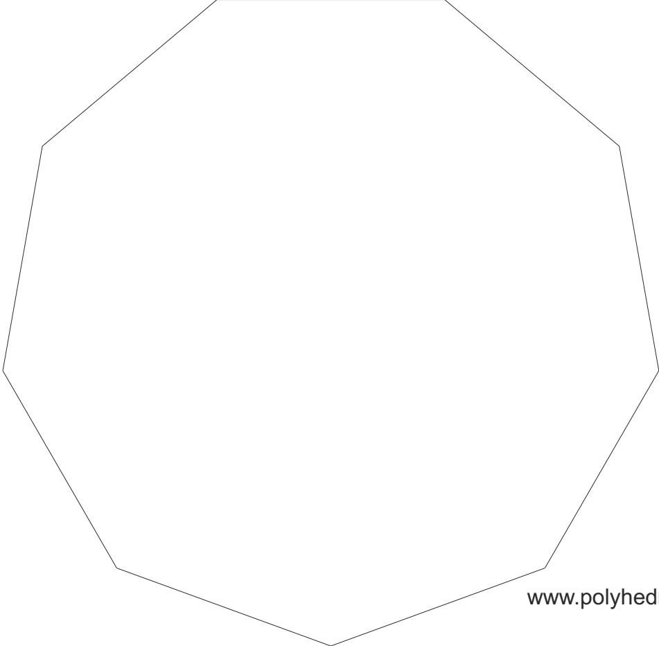
Enneagonal Pyramid
