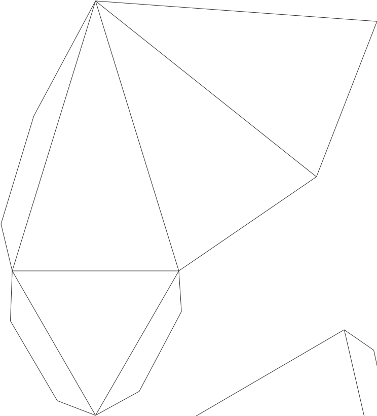
Triangular Pyramid
